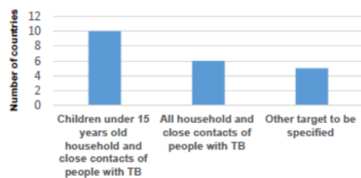
Figure 2: TPT Targets
